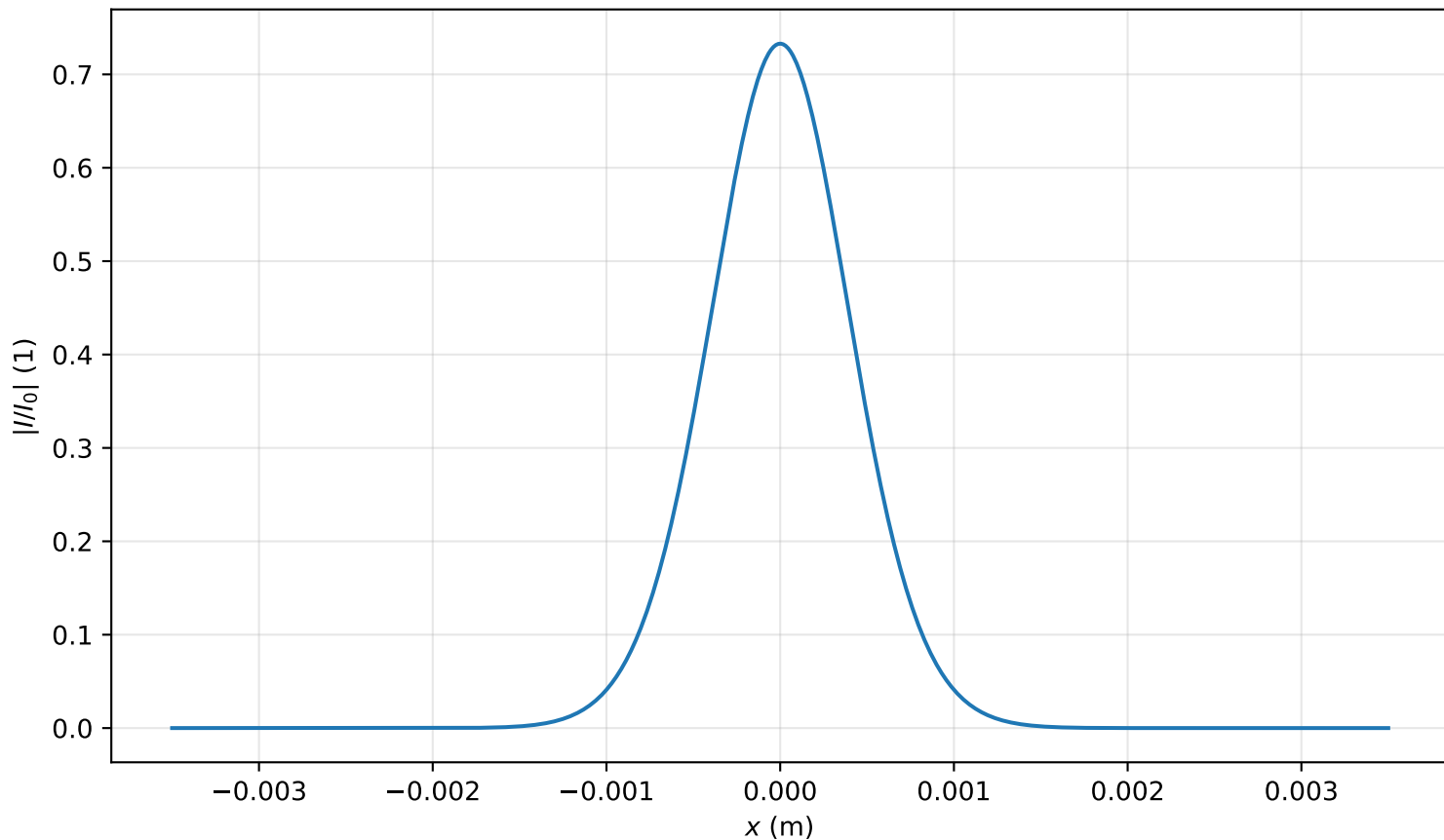
Intensity profile I(x, y = 0, z = 1.513m)/I_0 , P_{in}=0.2P_{cr} , artificial time
